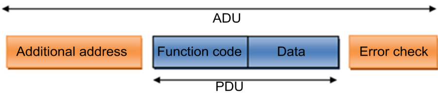
Figure 7-2 Modbus generic frame format
