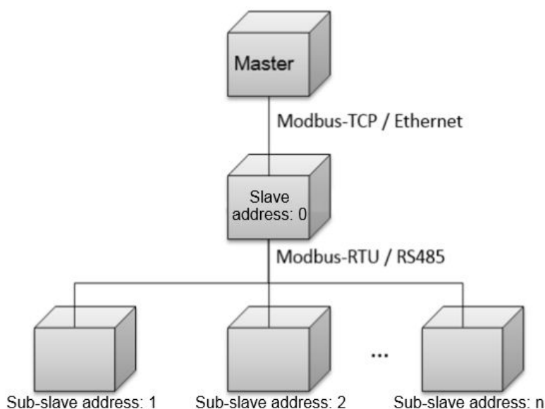
Figure 7-5 Communications address of the three-layer object structure
