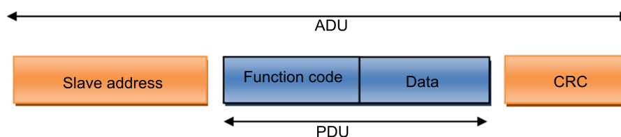
Figure 7-3 Modbus-RTU frame format
