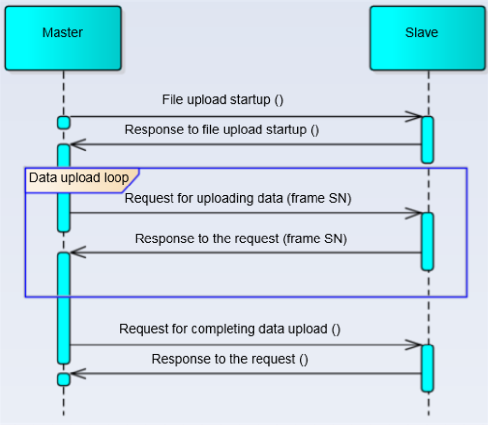
Figure 7-7 File uploading process
