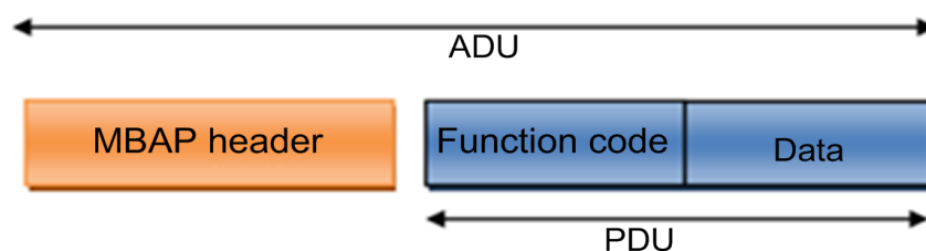
Figure 7-4 Modbus-TCP frame format
